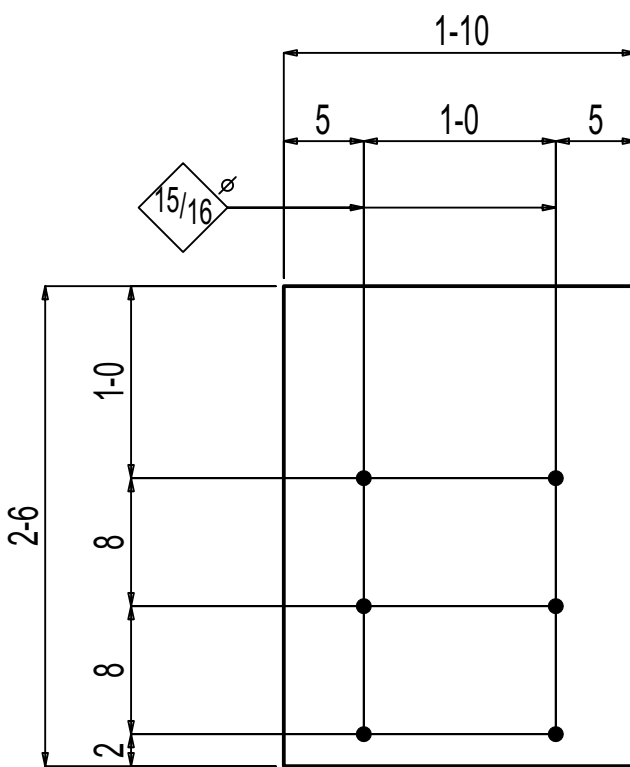
ONE EMBED PLATE F-11.03EP2
