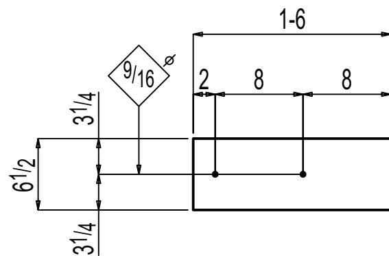
ONE LEVELING PLATE F-11.03LP2
