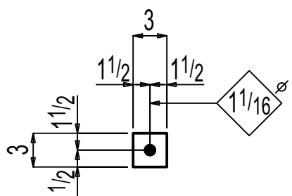
6 PLATE WASHERS F-11.03M10
