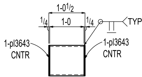
ONE HSS F-11.03M4
