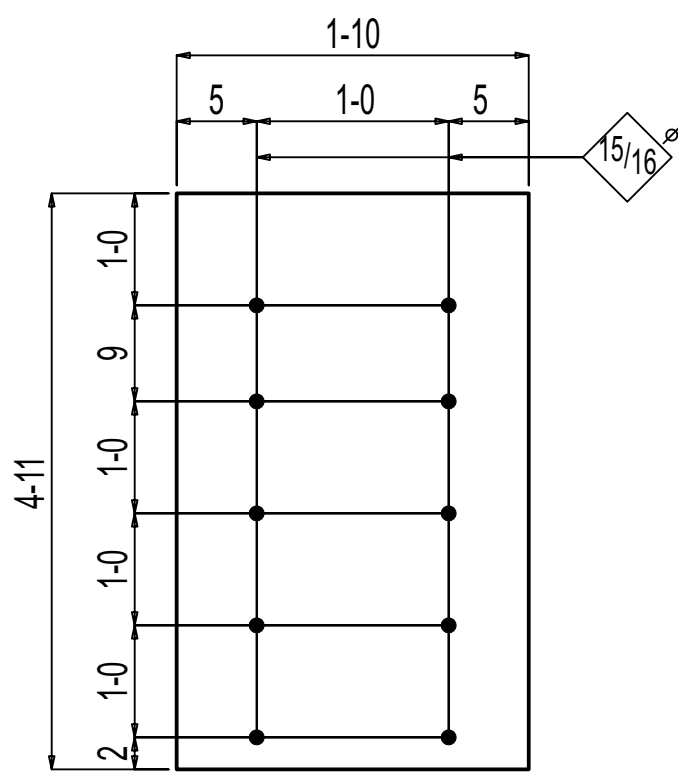
ONE EMBED PLATE F-11.03EP1
