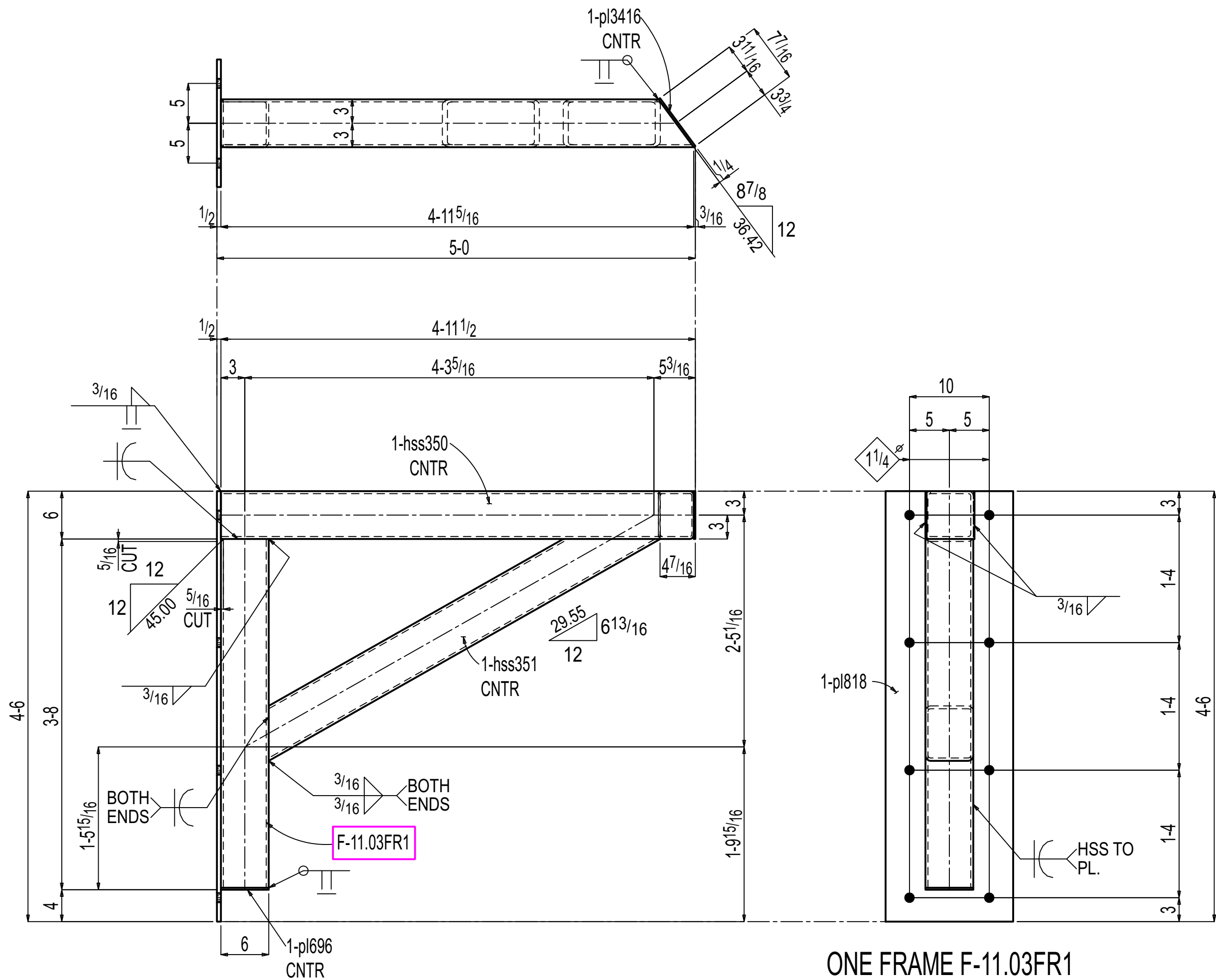
ONE FRAME F-11.03FR1
